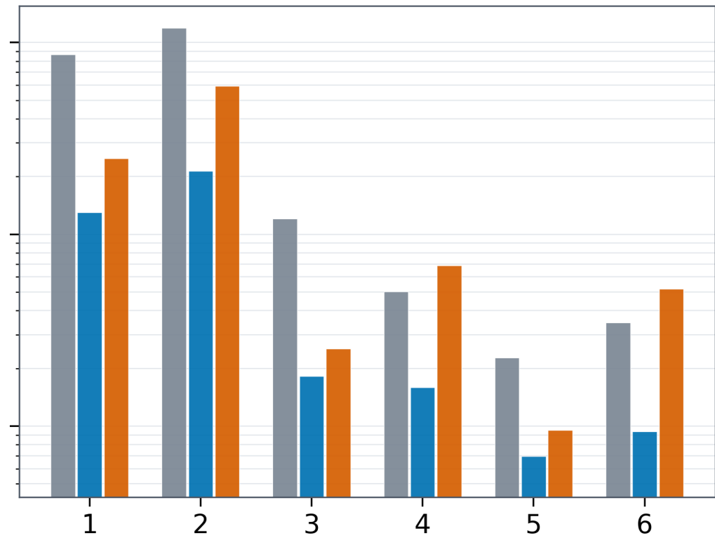
linear limb-darkened source
