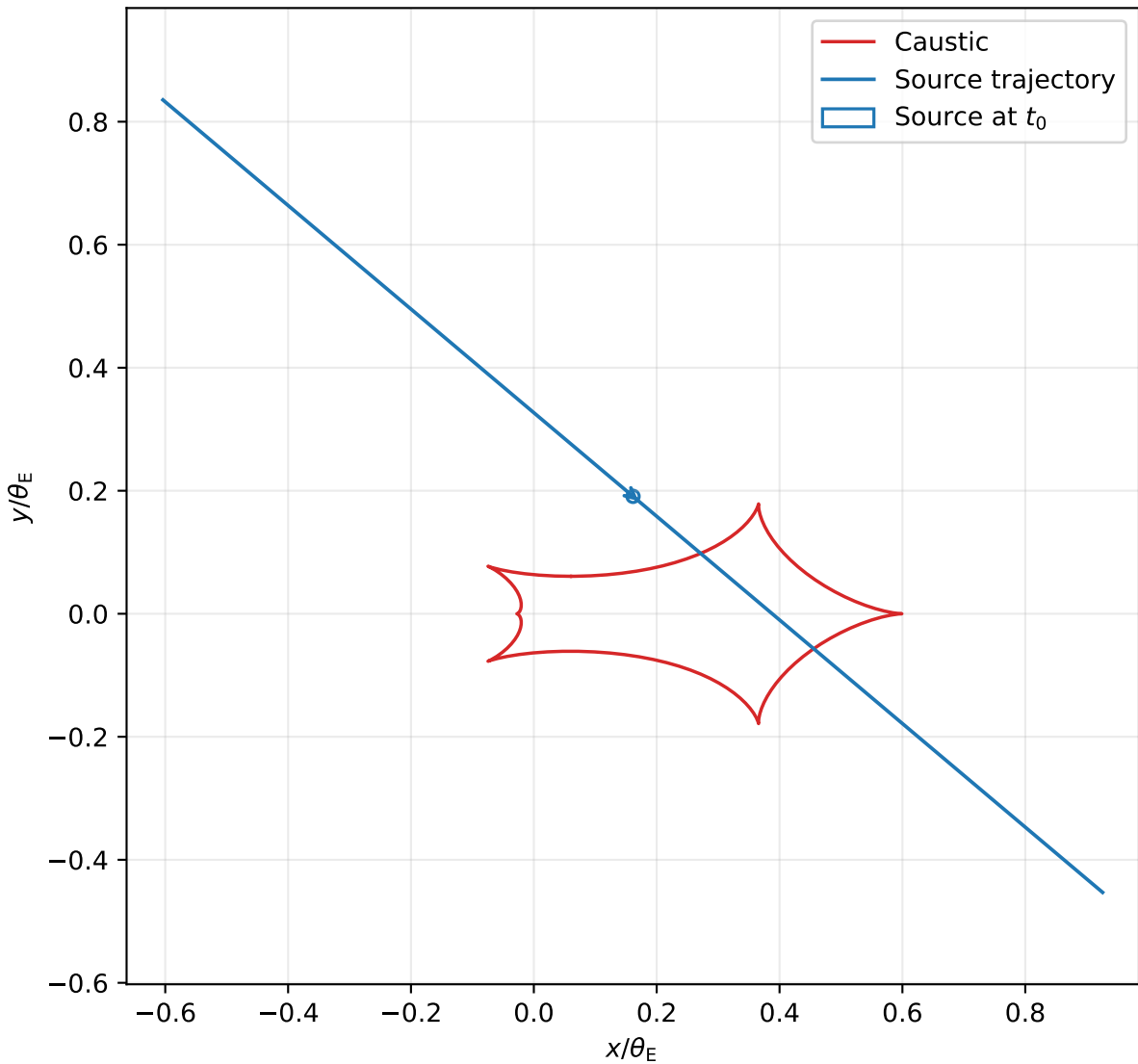
Binary lens caustics and source trajectory
