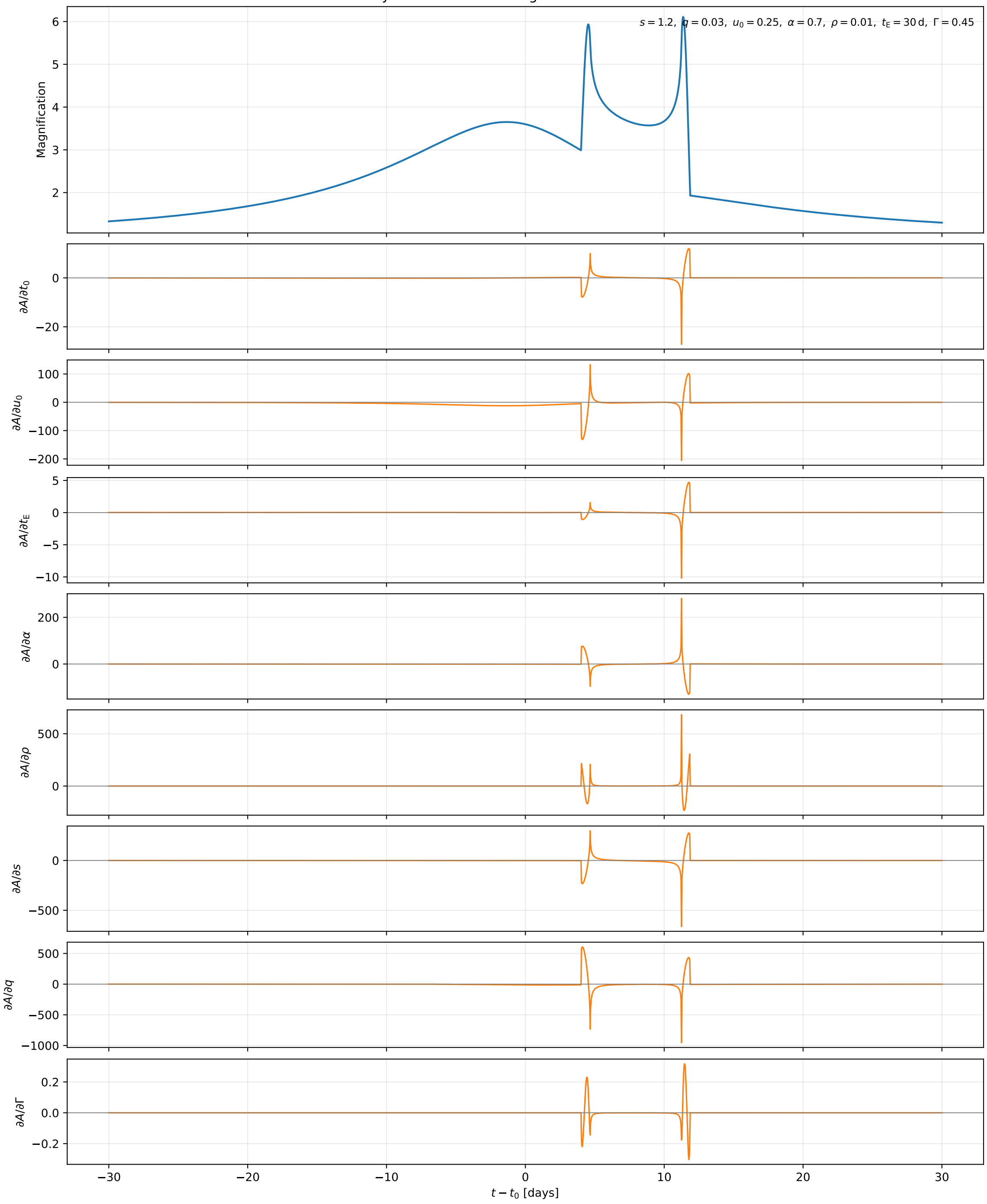
Binary lens: finite-source light curve and derivatives
