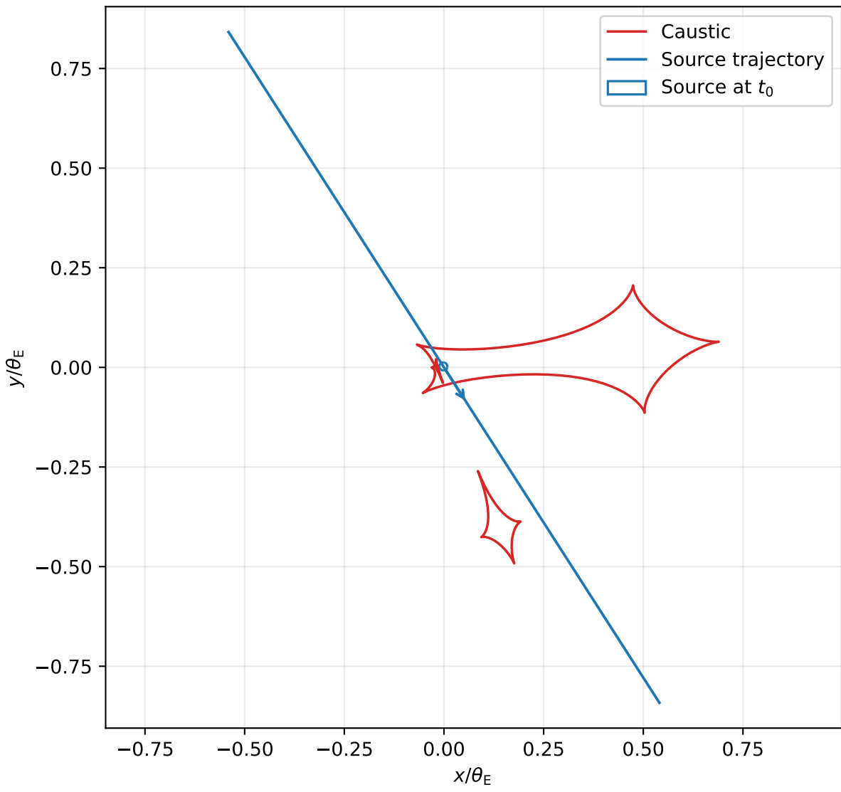
Triple lens caustics and source trajectory
