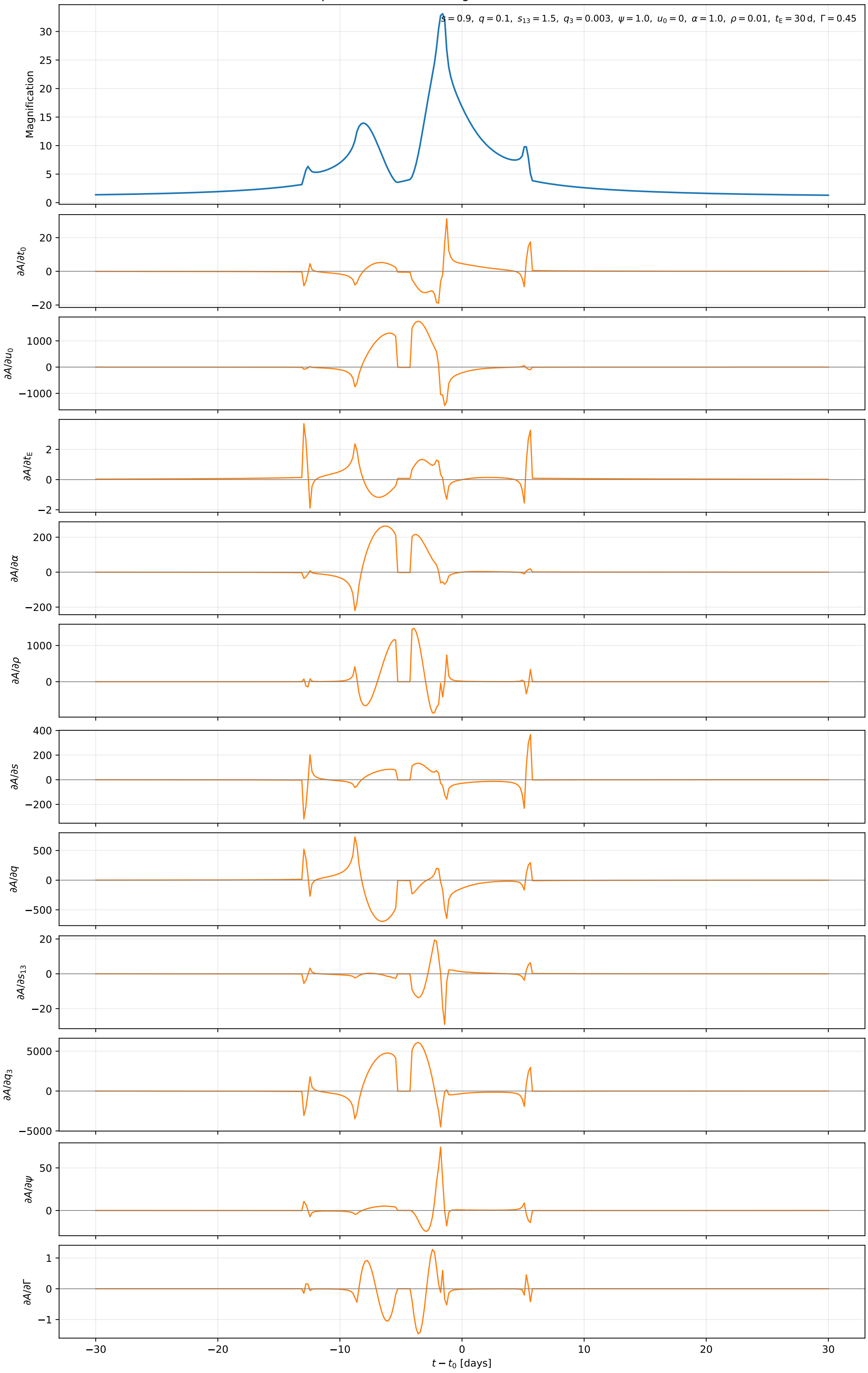
Triple lens: finite-source light curve and derivatives
