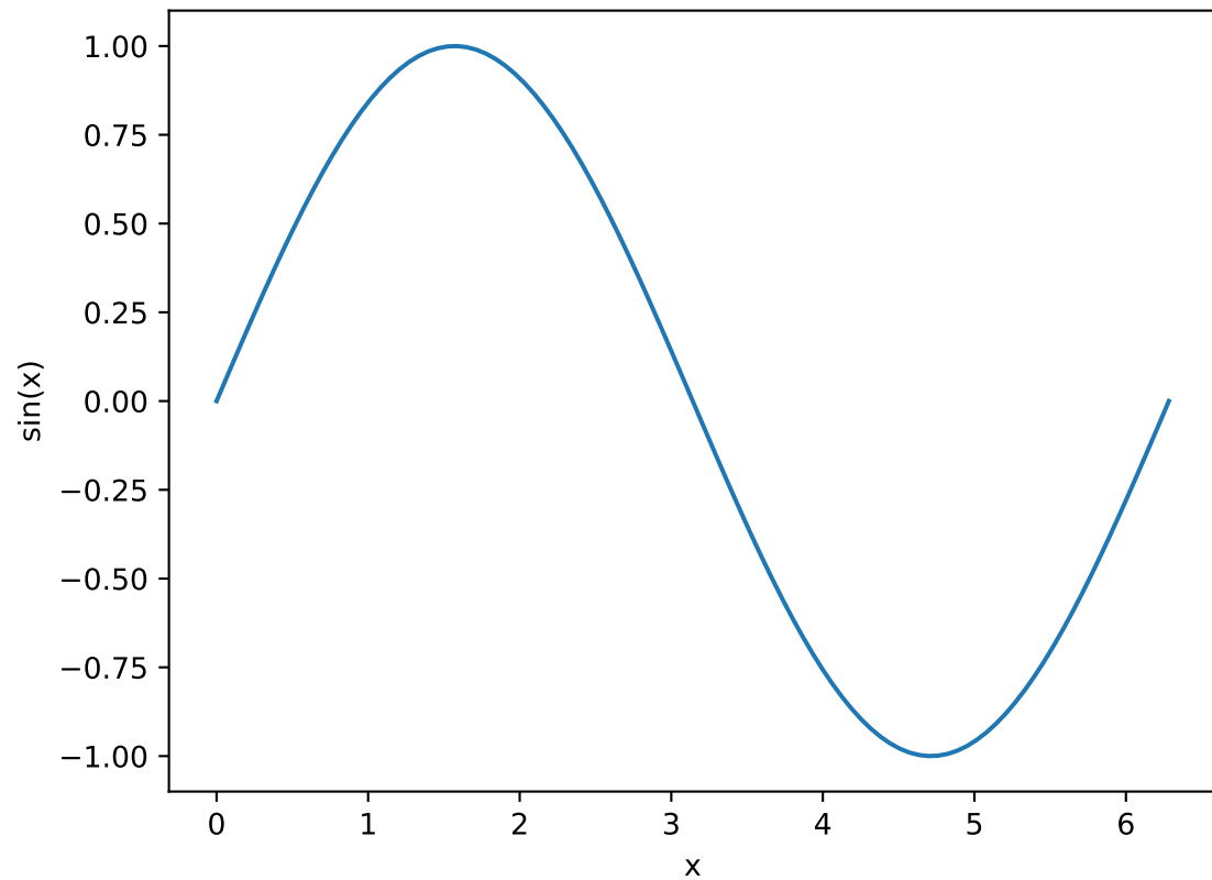
sin curve
