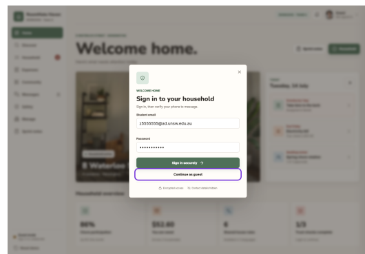
(b) Sprint 2: the visible focus indicator remains within the login dialog; Playwright verified the active element.
