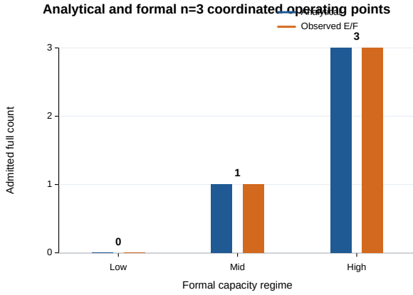
Fig. 2. Analytical and observed summary-preserving full-evidence counts.
