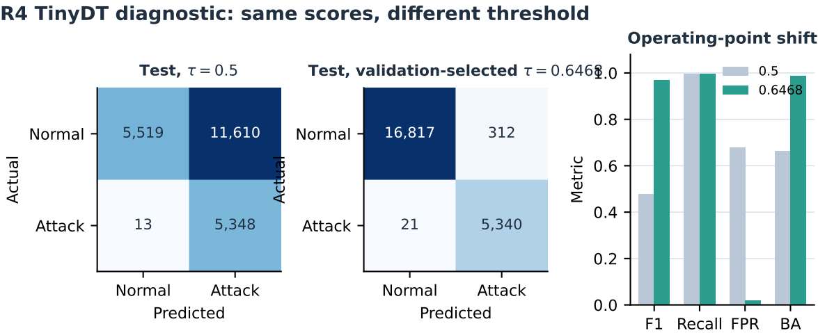
Figure S10. TinyDT threshold diagnostic. The primary threshold remains 0.5; the validation-selected threshold is a post-hoc diagnostic only.
