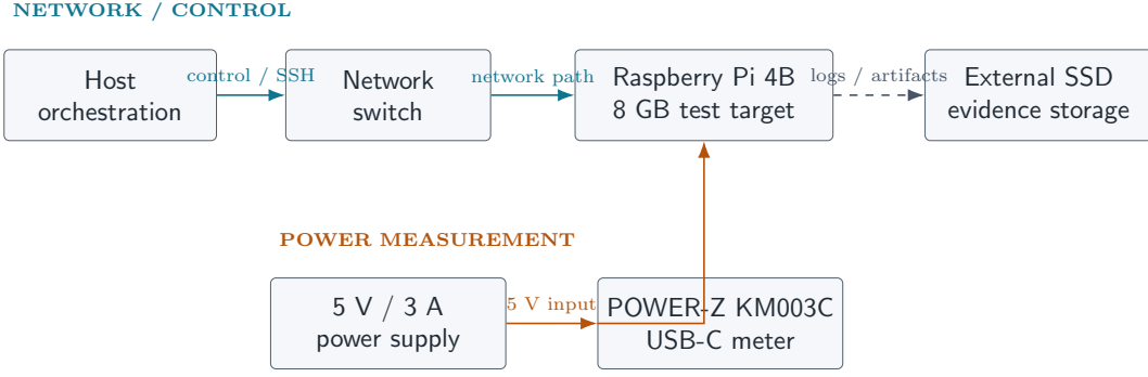
Fig. 1. Schematic apparatus overview. A 5-V supply feeds the Raspberry Pi 4B through the POWER-Z KM003C USB-C meter; network orchestration reaches the Pi via the switch; the external SSD stores evidence artifacts. The drawing shows roles and paths only.
