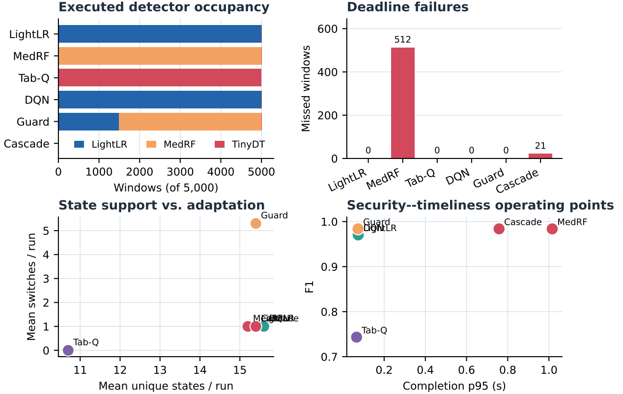
Fig. 2. R2 operational dashboard: realized detector occupancy, deadline misses, state support and switching, and security–timeliness operating points across the frozen 60-run factorial. DeadlineGuard is the single method with true load-conditioned switching and zero deadline misses; Tabular-Q’s TinyDT collapse under new load states is visible in the occupancy panel.
