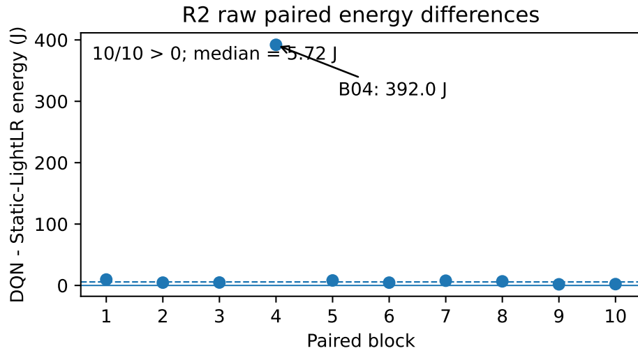
Figure S8a. R2 DQN-minus-Static-LightLR raw energy by paired block. Nine differences are between 1.8 and 9.6 J; Block 4 is a 392.0-J power/temperature excursion.
