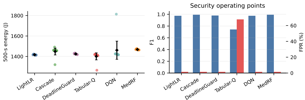
Figure S8. R2 raw energy distributions and security operating points. The block is the repeat unit.
