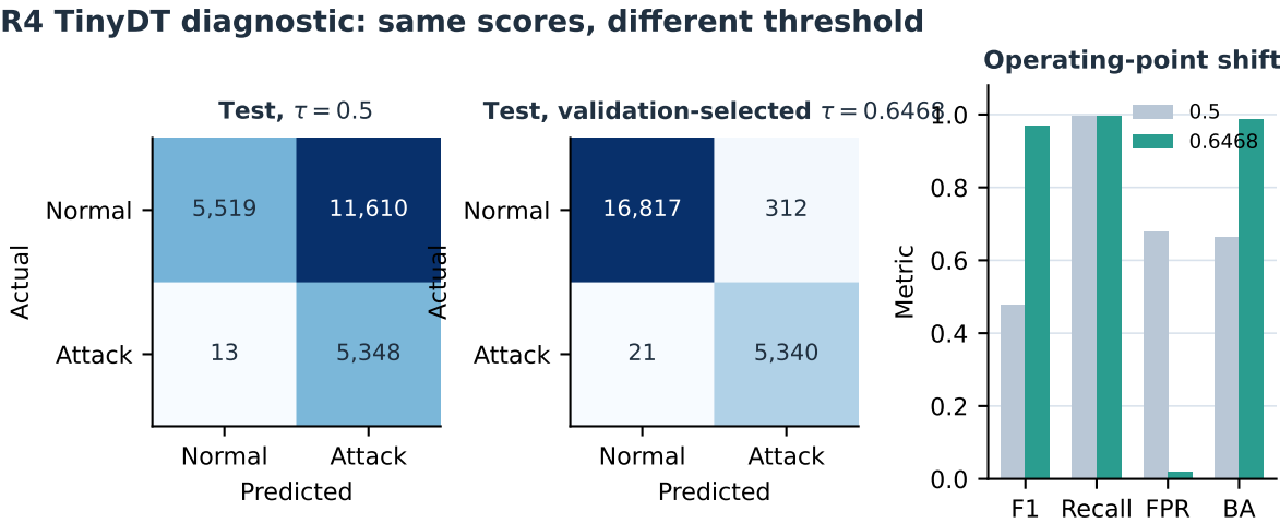
Figure S10. R4 TinyDT threshold diagnostic. The primary threshold remains 0.5; the validation-selected threshold is a post-hoc diagnostic only.
