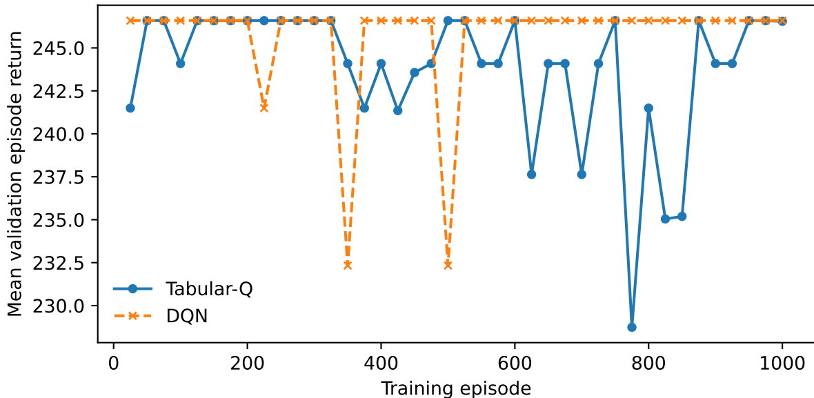
Validation every 25 episodes; selected checkpoints: Q 50, DQN 25
