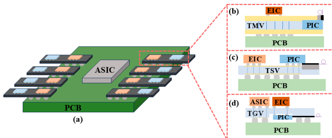
Figure 4. (a) Switch composed of 2.5D advanced packaging; (b) TMV-based, (c) TSV-based, and (d) TGV-based advanced packaging architectures.
