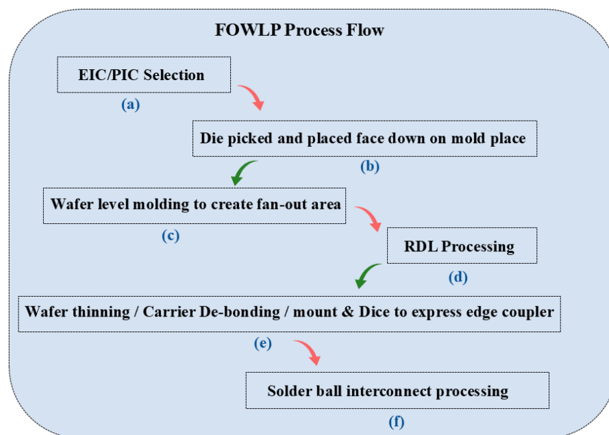
Figure 3. FOWLP process flow for OE packaging.
