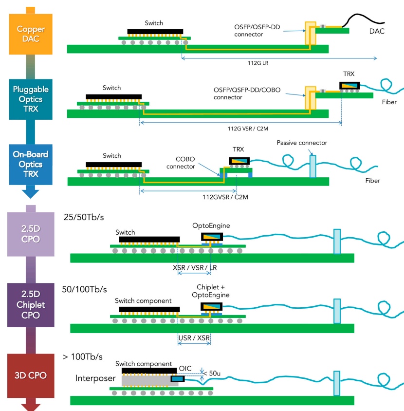
Figure 2. CPO packaging technology roadmap [59].
