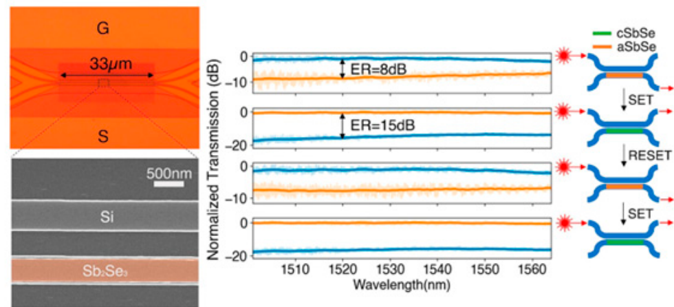
Figure 11. Electrical control of directional coupler switches [183].
