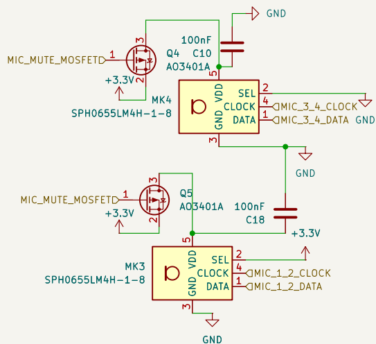
Microphones 3-4
