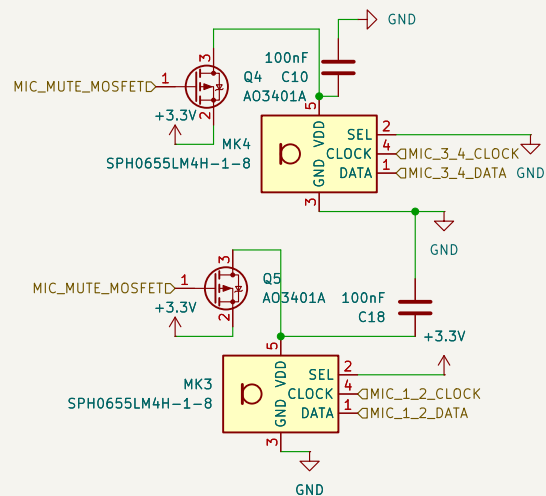
Microphones 3-4
