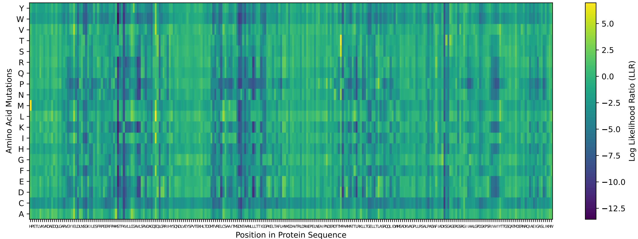
Predicted Effects of Mutations on Protein Sequence (LLR)
