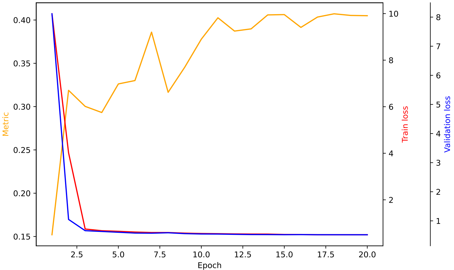
Training History
