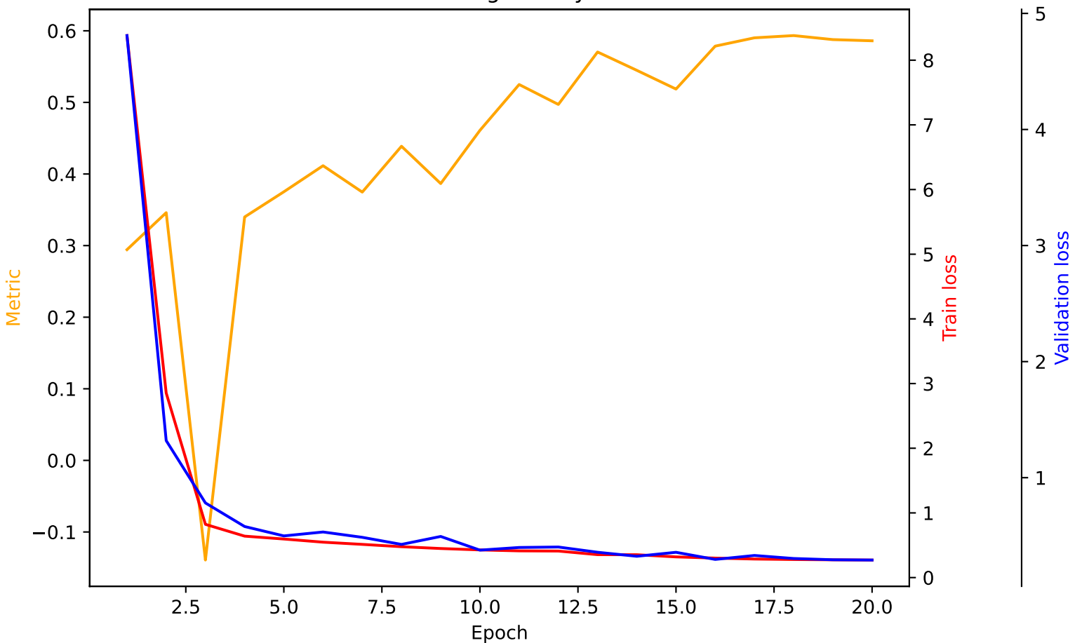
Training History
