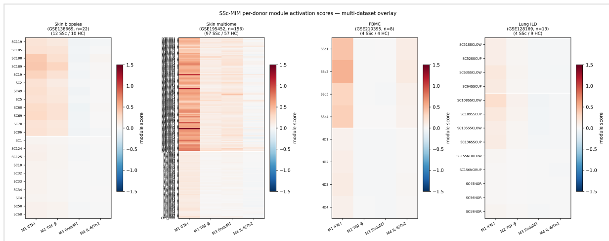
Figure 2: Multi-tissue single-cell transcriptomic overlay of SSc-MIM. Four-panel heatmap of per-donor module activation scores (M1–M4) across skin biopsies (GSE138669, n=22), skin multiome (GSE195452, n=156), PBMC (GSE210395, n=8), and lung ILD (GSE128169, n=13) donors, stratified by SSc vs HC. Generated as `figures/F2_multi_overlay.svg`.
