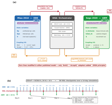
Fig. 1. OISA workflow for the influenza coupling reference implementation. (a) Architecture diagram: Miao 2010 ODE (SBML, BIOMD0000000546) and Sego 2020 CC3D ABM (CompuCell3D 4.8.0, GitHub @5b7e42c) connected through the OISA Orchestrator, with ISSL signal arrows annotated with signal_id and biological units. (b) GSimT timeline for a representative 5-day window: ODE ticks every 6h, ABM ticks every 24h = 72 MCS, ISSL checkpoints (orange dots), and causal-ordering annotation (ABM.emit \rightarrow ODE.accept \rightarrow ODE.step \rightarrow ODE.emit) at the 24h boundary.
