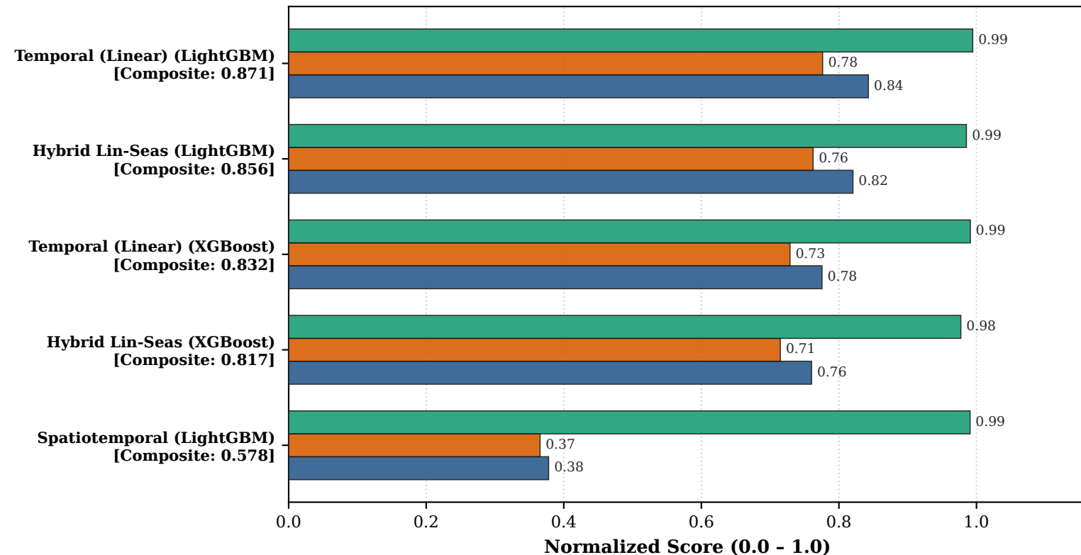
(b) MAR Scenario: Top-5 Combinations
