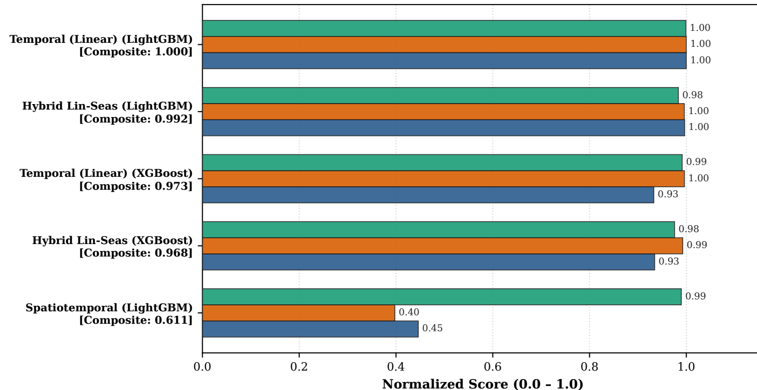
(a) MCAR Scenario: Top-5 Combinations
