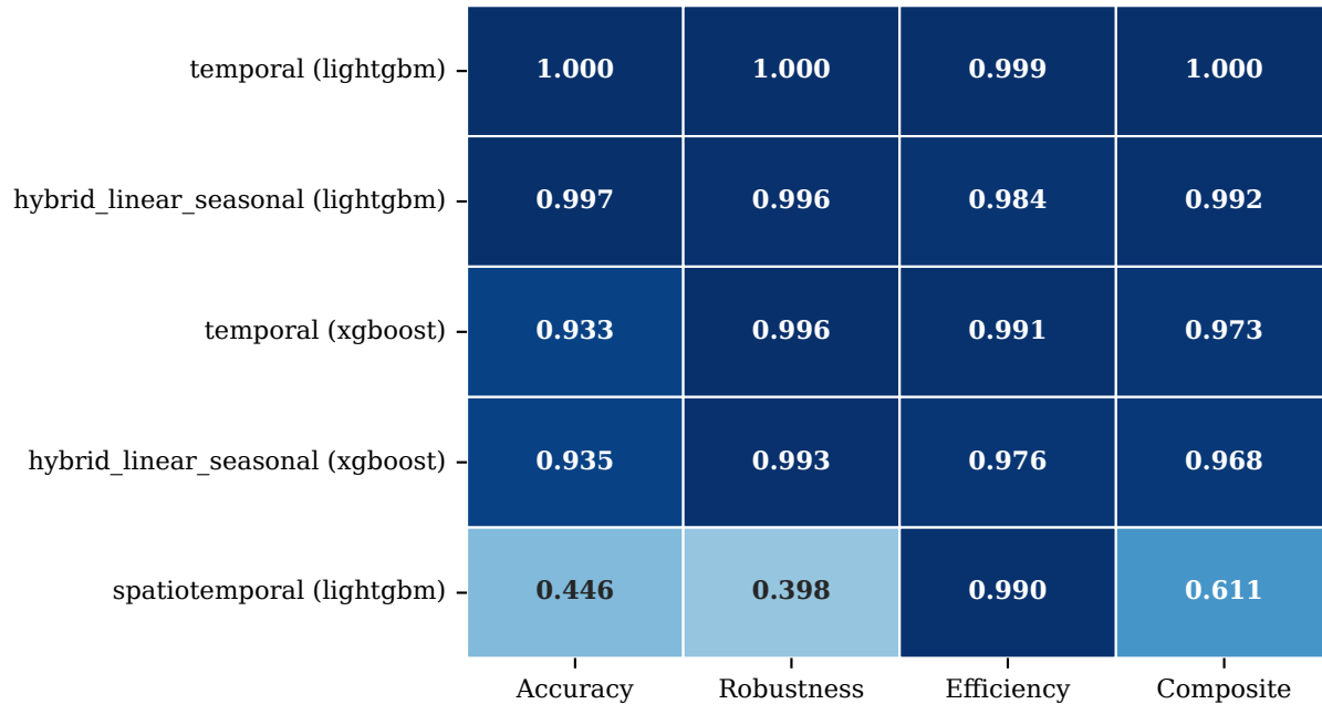
(a) MCAR Scenario: Top-5 Performance Matrix
