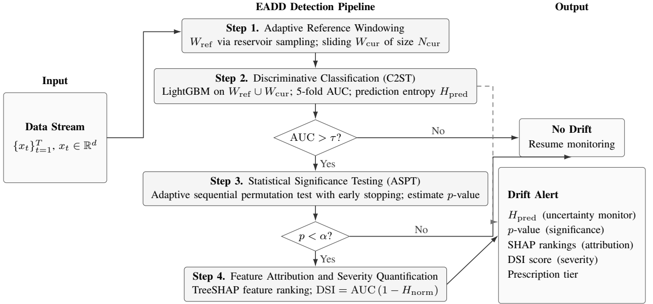
Fig. 1. EADD detection pipeline. W_{cur} is compared against W_{ref} via a discriminative classifier; H_{pred} provides a continuous uncertainty monitoring signal (dashed). AUC > \tau triggers ASPT for statistical confirmation (Step 3); upon significance, TreeSHAP and DSI localise and quantify the shift (Step 4).
