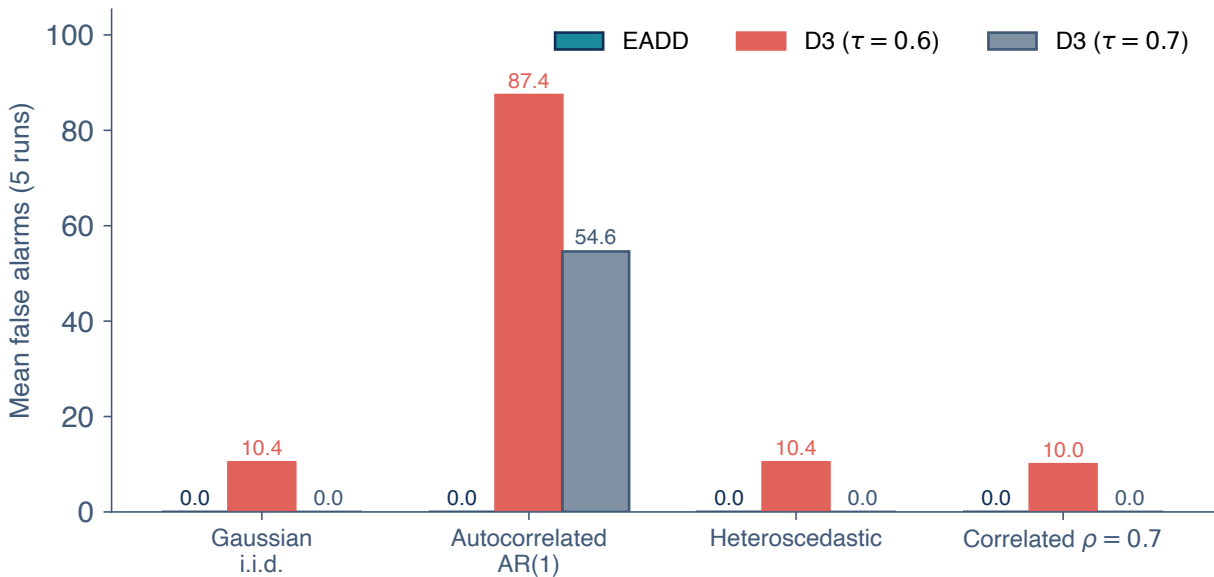
False-alarm robustness on stable (no-drift) streams
