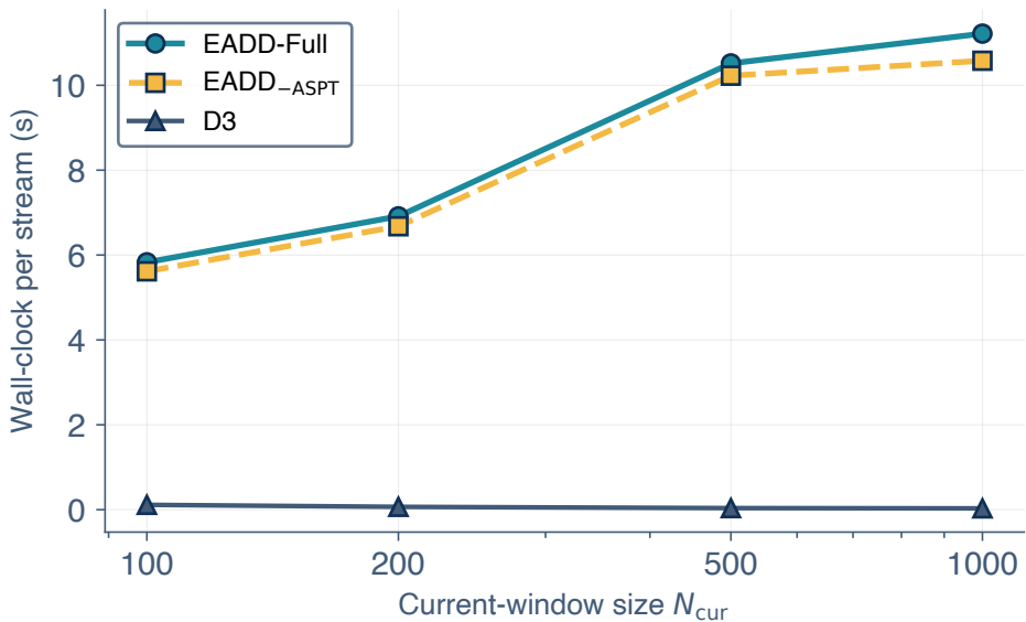
Wall-clock scaling with window N_{\text{cur}}
