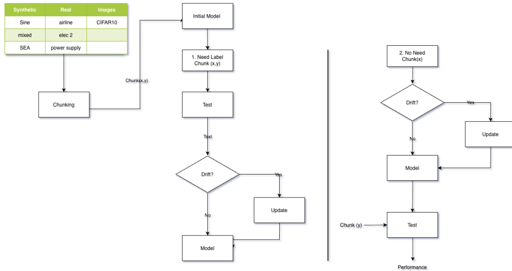
Figure 3.1: Overview of the proposed adversarial validation framework for feature drift detection.
