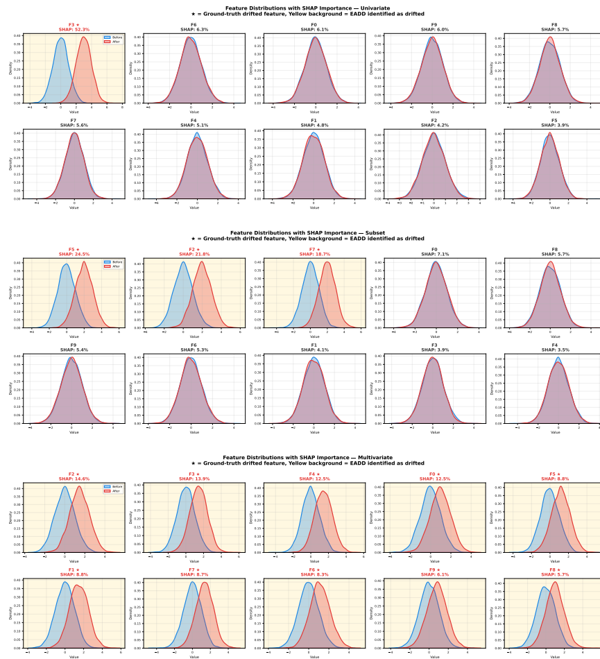
Figure 4.7: Combined bell curve and SHAP attribution analysis for three controlled scenarios. Top: Univariate drift—F3 dominates at 52.3%. Middle: Subset drift—F5, F2, F7 collectively account for 65%. Bottom: Multivariate drift—importance distributed evenly, max 14.6%.
