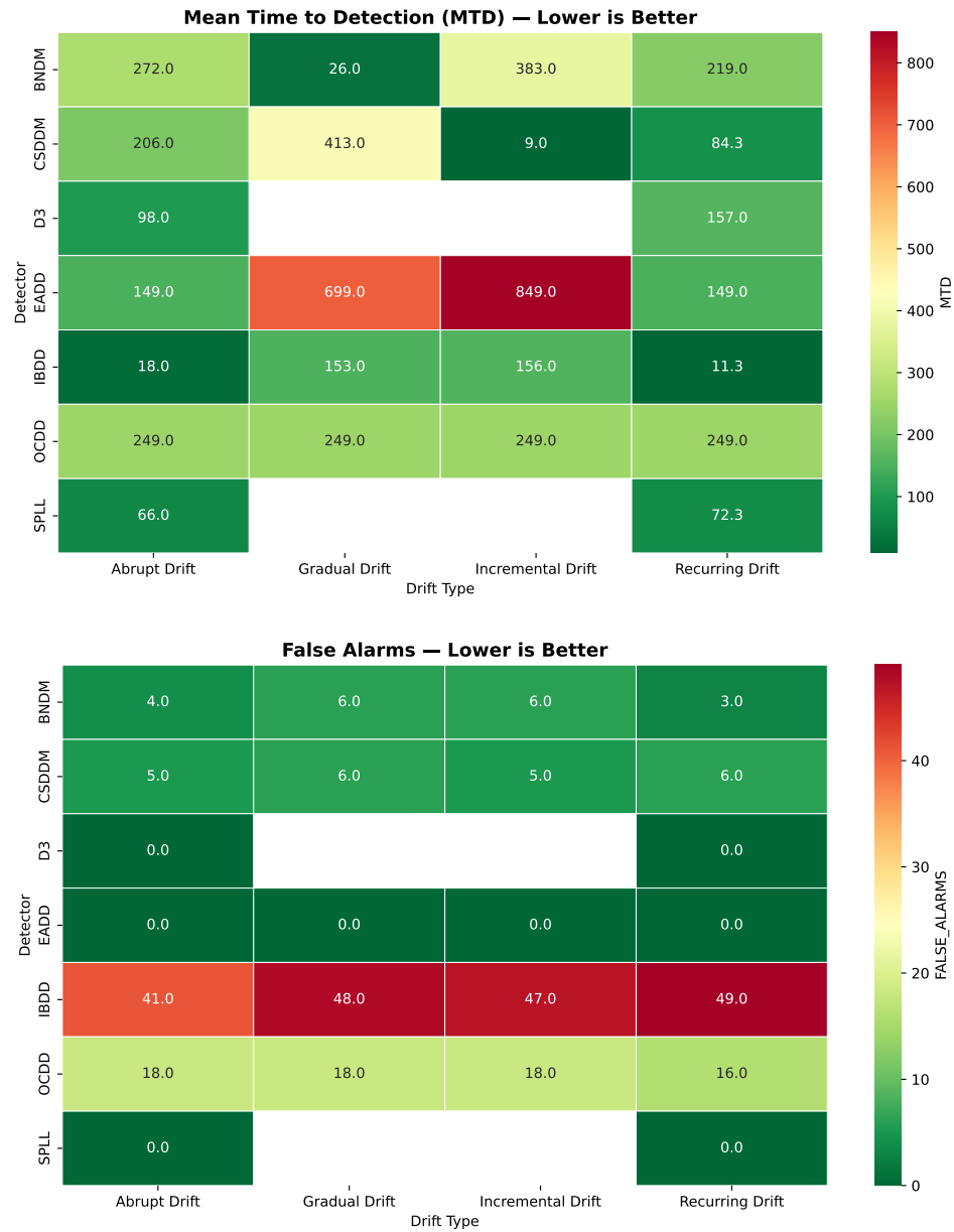
Figure 4.1: Heatmaps of detection performance on synthetic drift. Top: Mean Time to Detection (lower is better; white cells indicate complete miss). Bottom: False Alarm count (lower is better).
