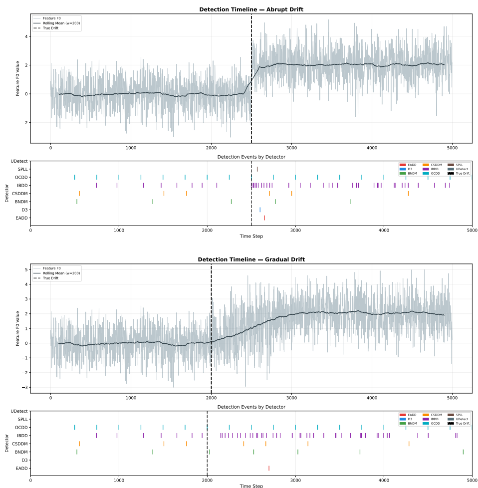
Figure 4.3: Time-series comparison of all eight detectors. Top: Abrupt drift—most detectors respond near the true drift point (dashed line). Bottom: Gradual drift—only EADD, BNDM, CSDDM, IBDD, and OCDD detect the shift; D3, SPL, and UDetect remain silent.
