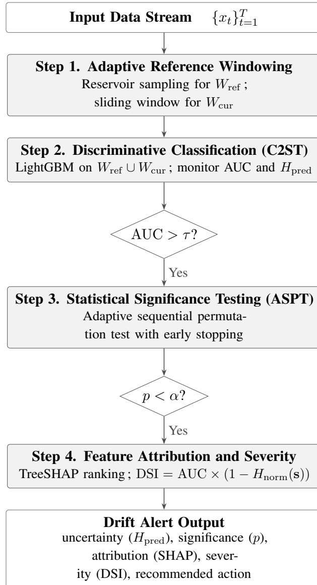
Figure 3.2: Detailed architecture of the Enhanced Adversarial Drift Detection (EADD) methodology, matching the pipeline design used in the JCSEE paper: adaptive windowing, discriminative detection, ASPT significance gating, and SHAP+DSI diagnostics.
