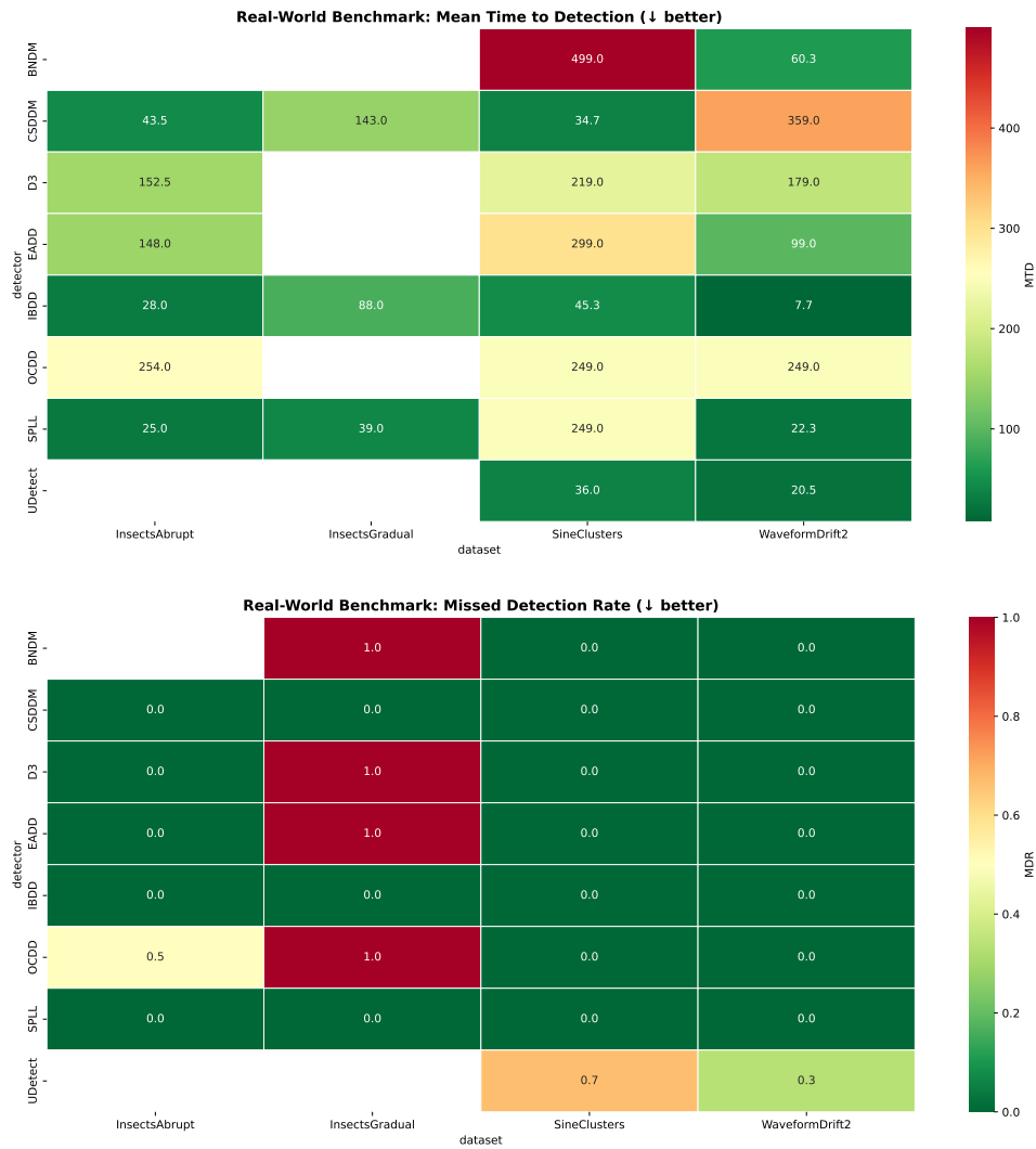
Figure 4.4: Heatmaps of real-world benchmark performance. Top: Mean Time to Detection (lower is better; white cells indicate missed drifts or timeout). Bottom: Missed Detection Rate (0.0 is perfect).
