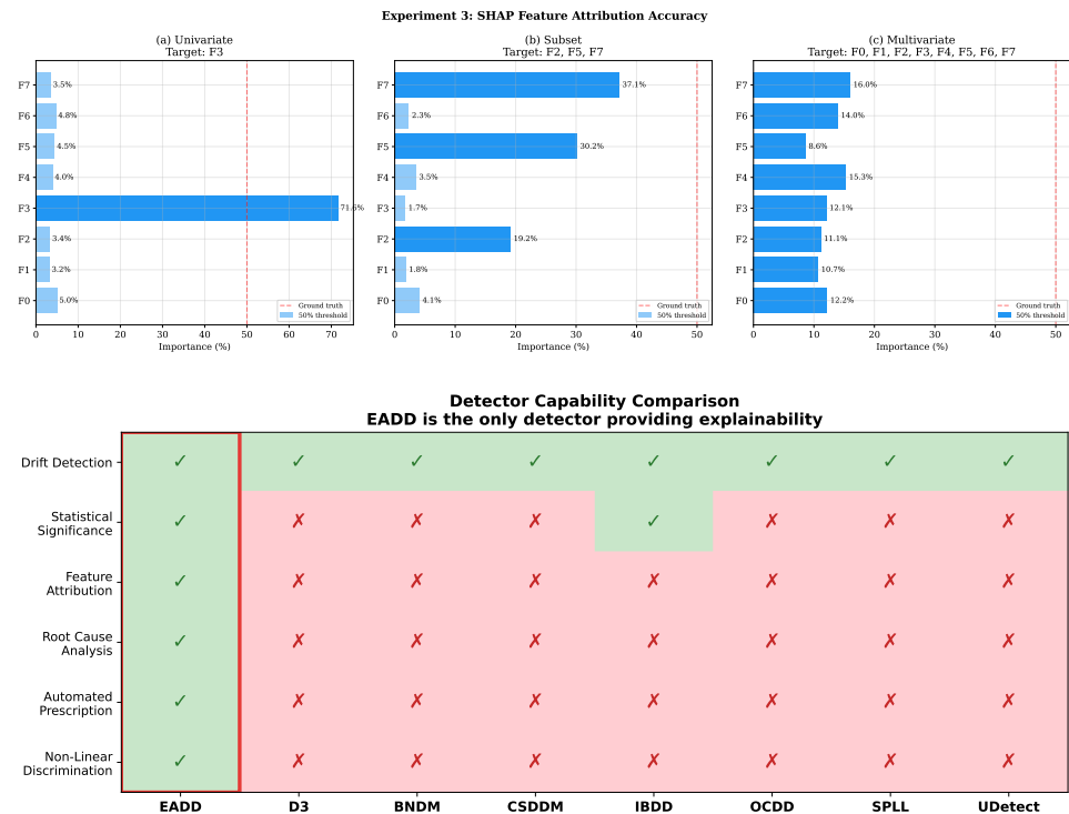
Figure 4.8: Top: SHAP attribution accuracy across all three scenarios ( P@k = R@k = F1@k = 1.0 for all). Bottom: Diagnostic capability comparison—EADD is the only detector providing feature-level attribution and automated prescriptions.
