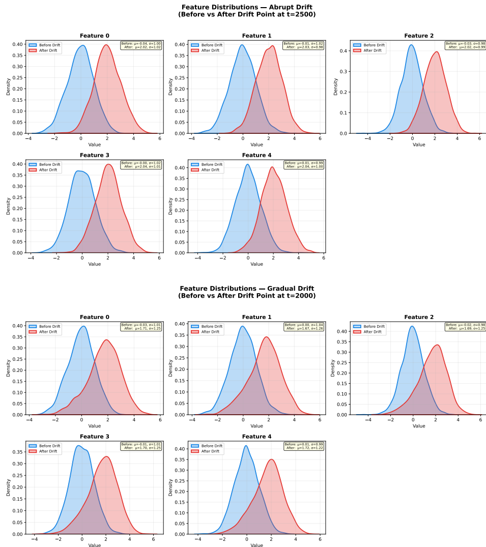
Figure 4.2: Bell curves showing feature distributions before (blue) and after (red) drift injection. Top: Abrupt drift with clear separation. Bottom: Gradual drift with overlapping distributions—the subtle shift that D3, SPL, and UDetect all failed to detect.
