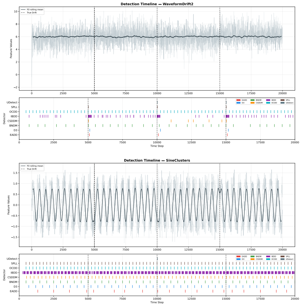
Figure 4.5: Time-series comparison on benchmark datasets from the multi-detector supplementary run. Top: WaveformDrift2 (semi-synthetic)—EADD detects all three drift points (MTD=99), outperforming D3 (MTD=179). Bottom: SineClusters (semi-synthetic)—IBDD detects rapidly but with many excess detections, illustrating the sensitivity–specificity trade-off.
