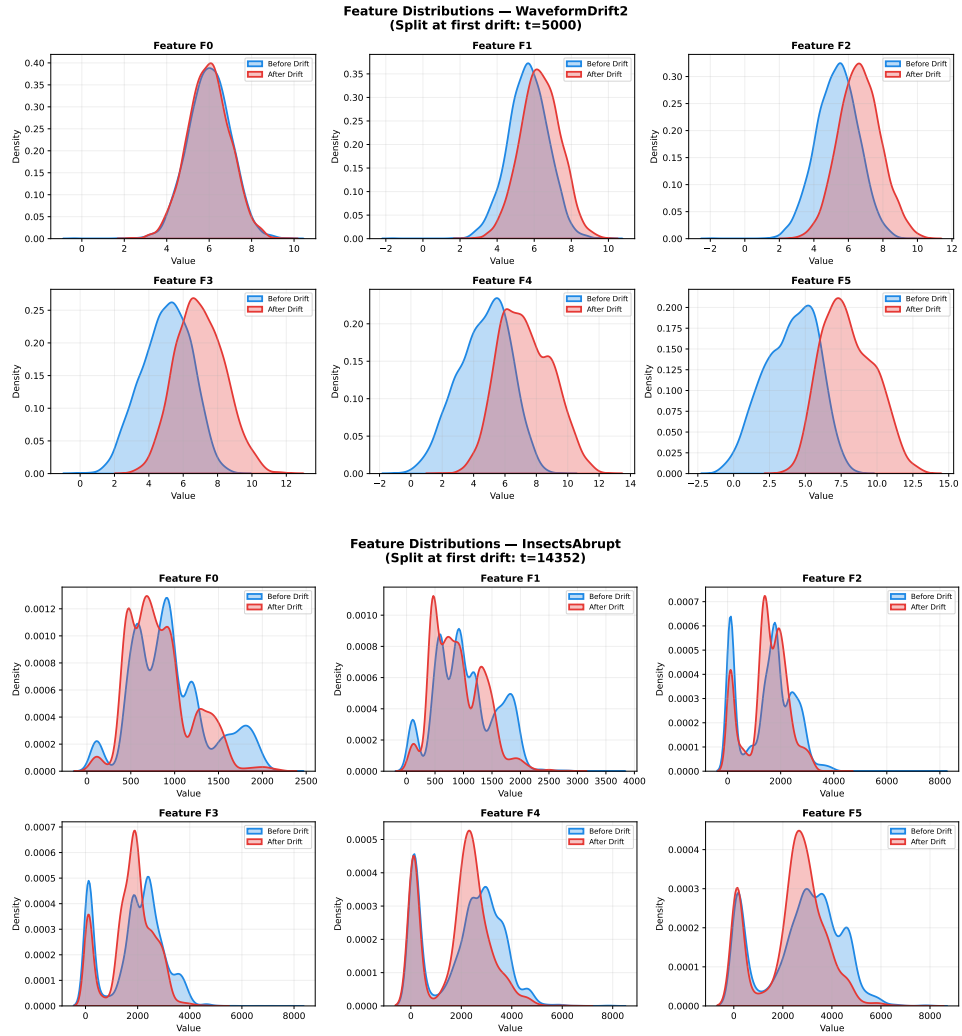
Figure 4.6: Feature distribution bell curves. Top: WaveformDrift2 (semi-synthetic) showing multi-dimensional distributional shift across 21 features. Bottom: InsectsAbrupt showing abrupt distributional changes across 33 features.
