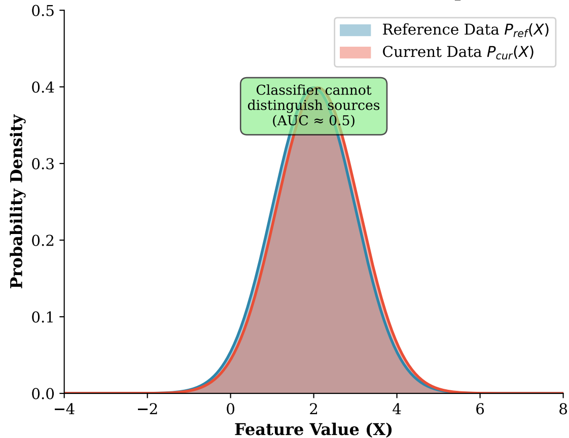
No Drift: Distributions Overlap
