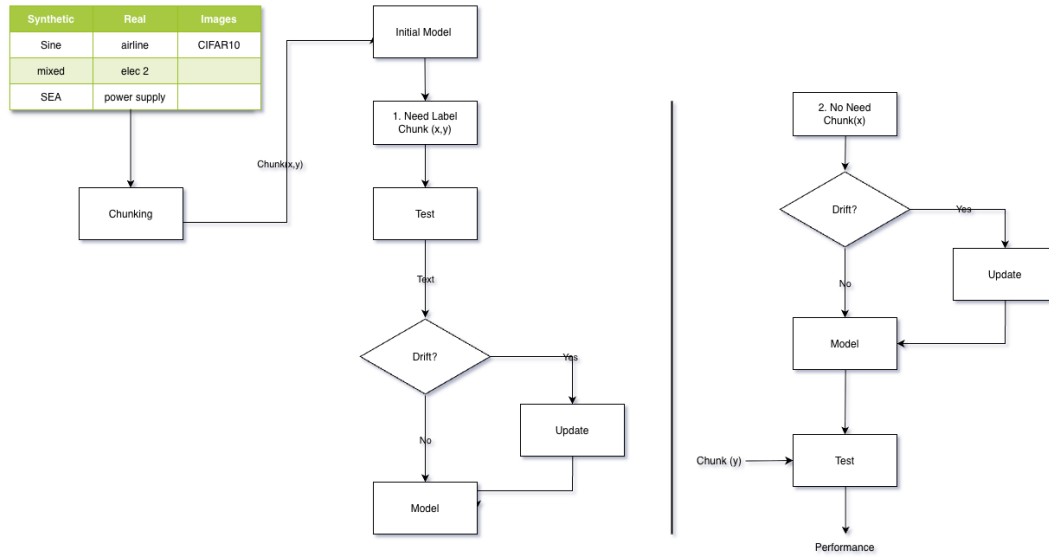
Figure 3.2: Overview of the proposed adversarial validation framework for feature drift detection.
