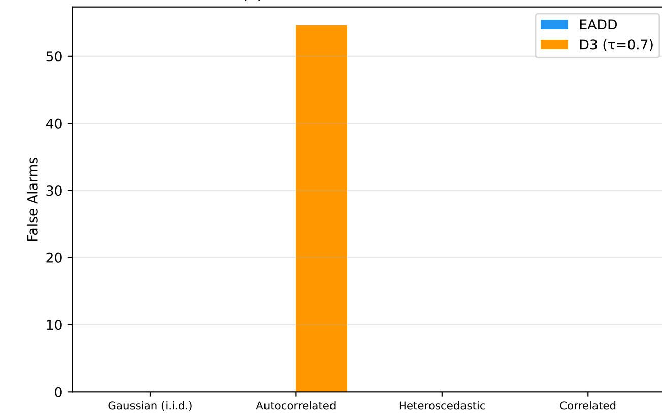
(c) False Alarms on Stable Data
