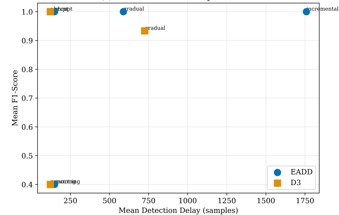
(c) F1 vs Detection Delay Trade-off
