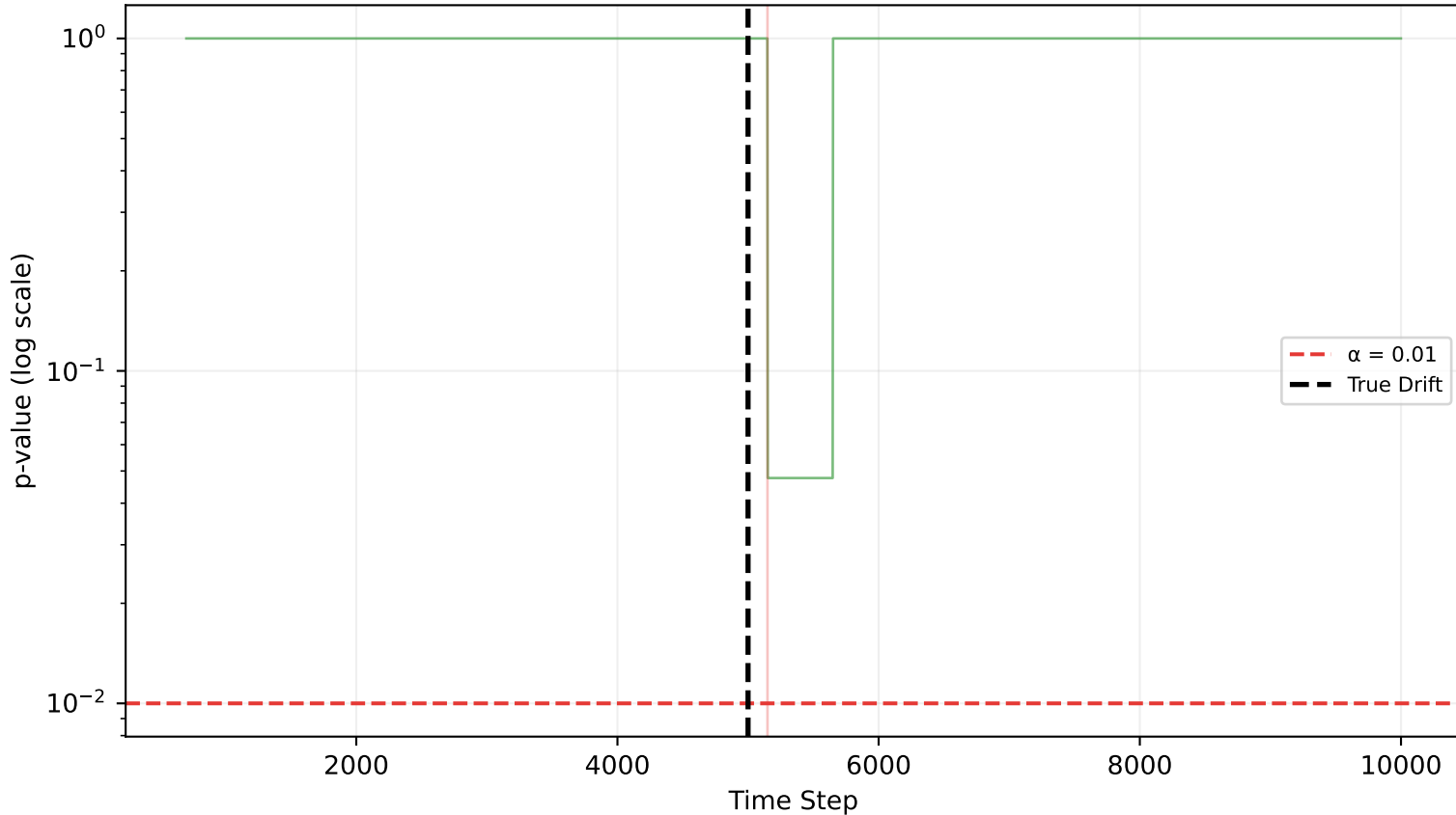
Stage 2: Permutation p-value
