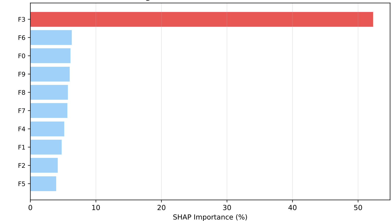
Stage 3: SHAP Feature Attribution
