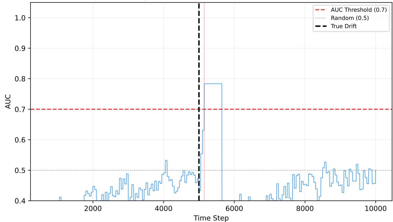
Stage 1: Adversarial AUC Over Time
