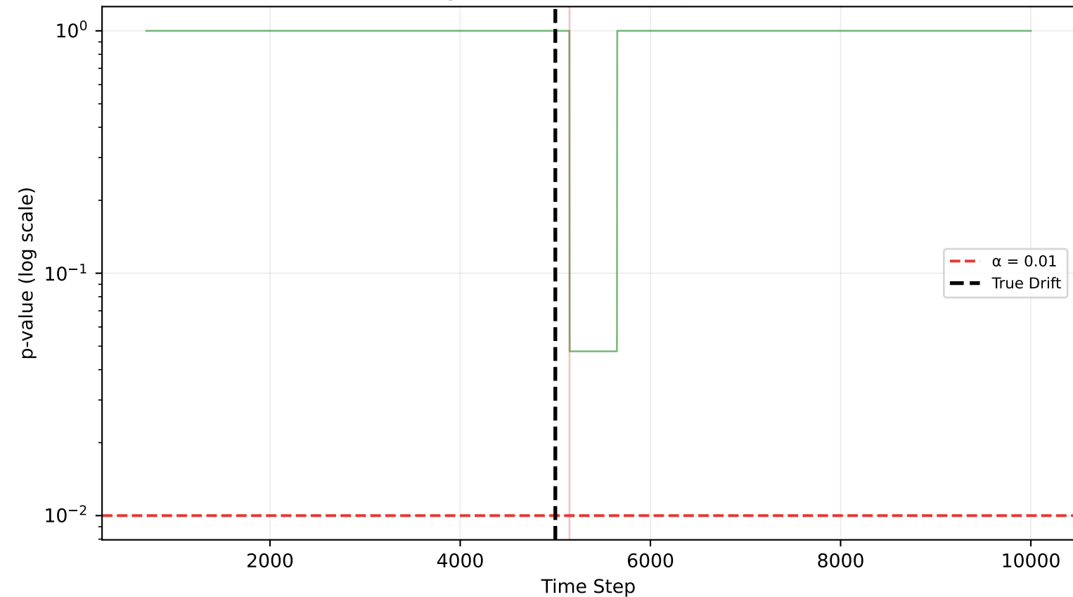
Stage 2: Permutation p-value
