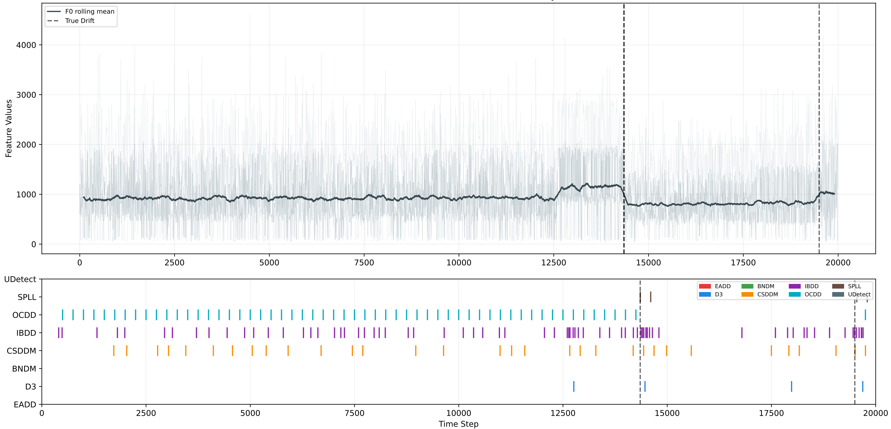
Detection Timeline — InsectsAbrupt
