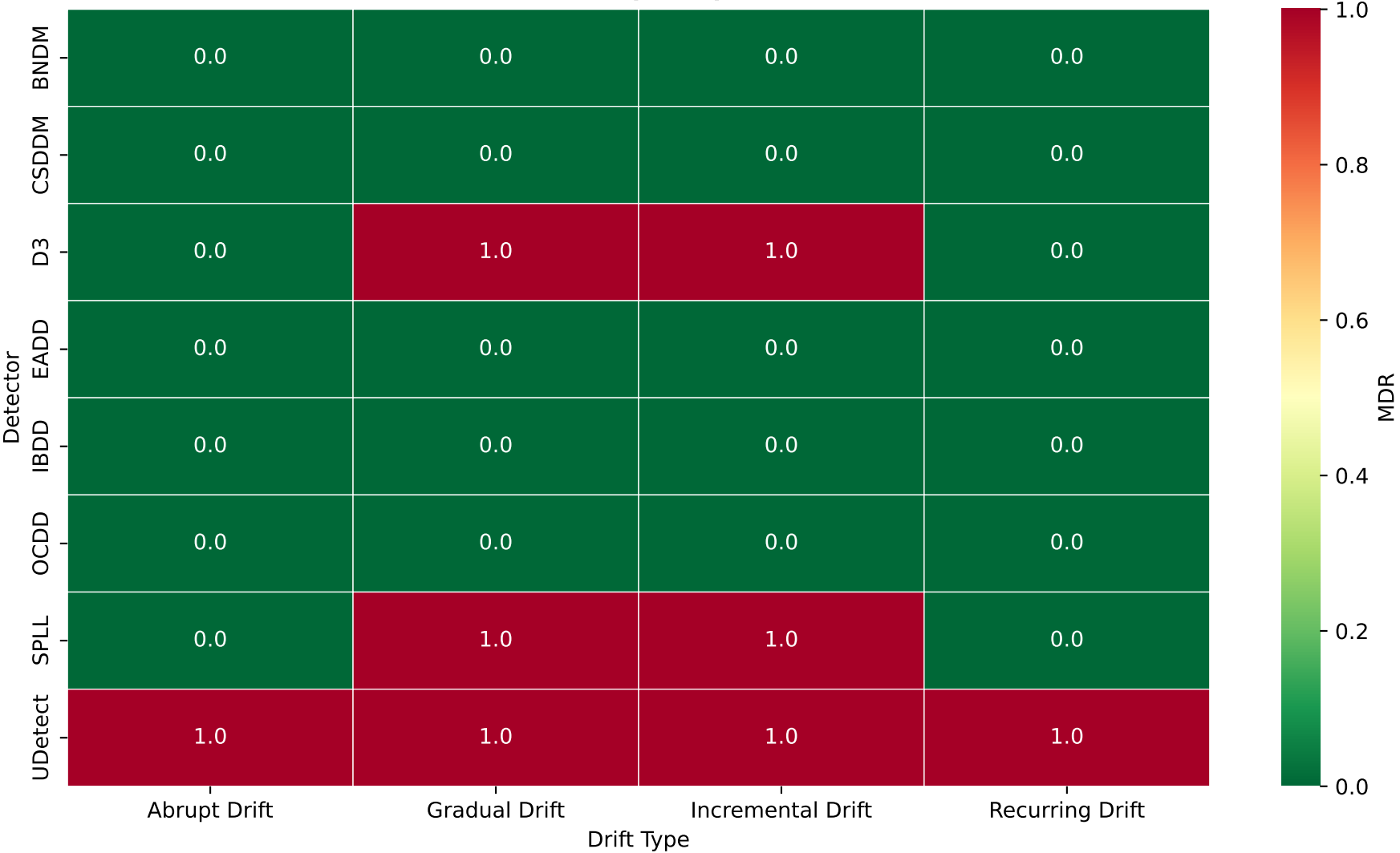
Missed Detection Rate (MDR) — Lower is Better
