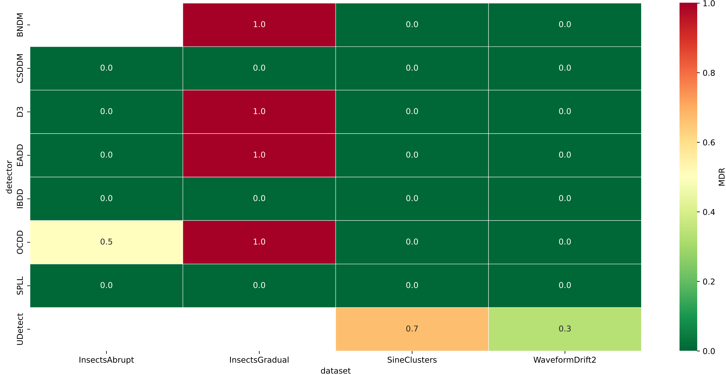
Real-World Benchmark: Missed Detection Rate (↓ better)
