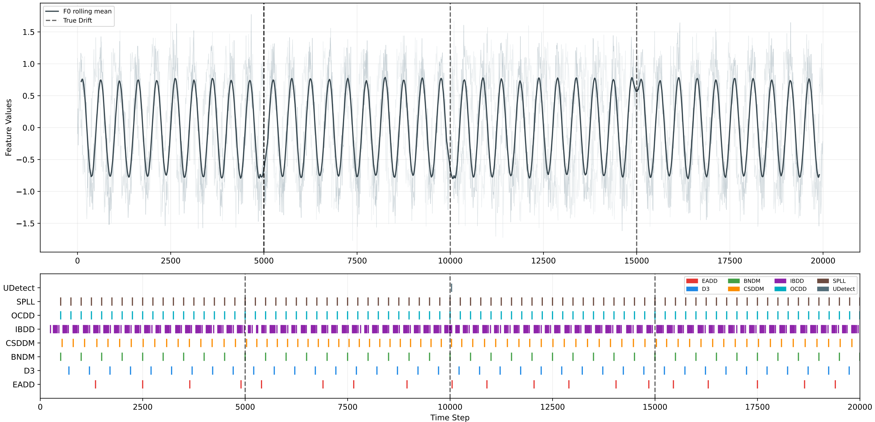
Detection Timeline — SineClusters
