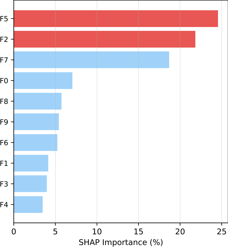
Stage 3: SHAP Feature Attribution
