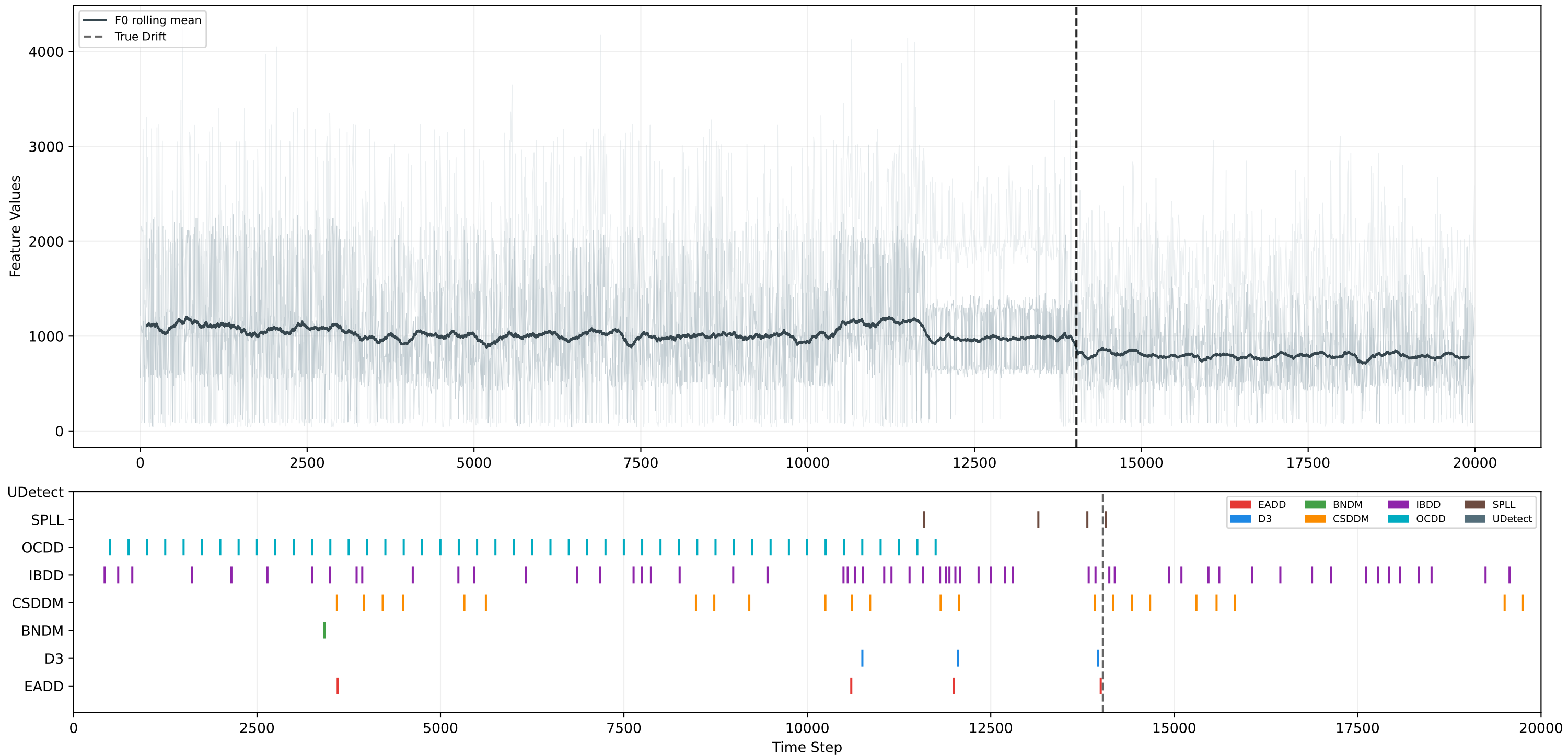
Detection Timeline — InsectsGradual
