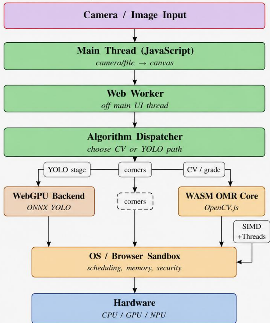
(a) Layered Runtime Model
