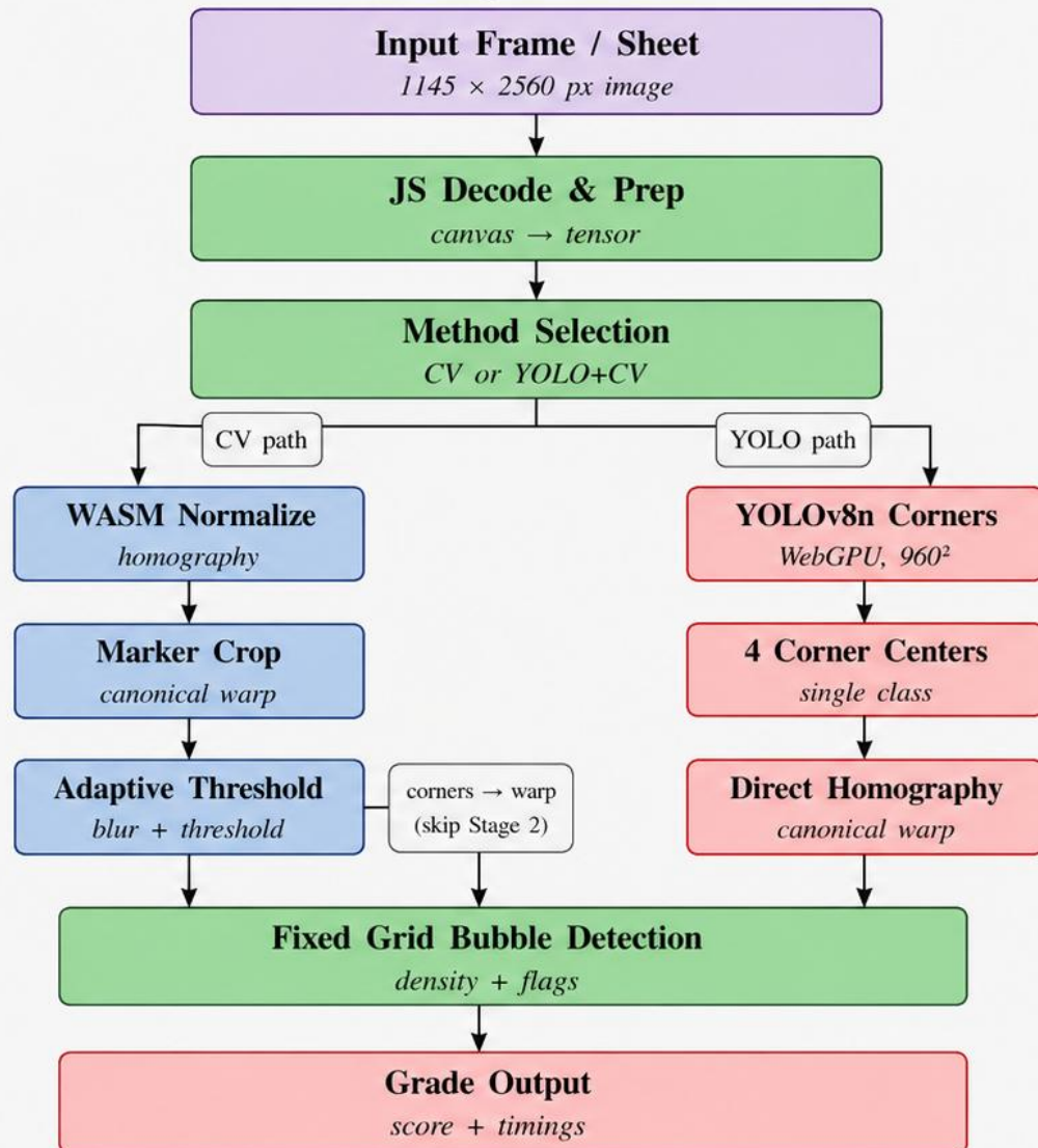
(b) Algorithm Flow
