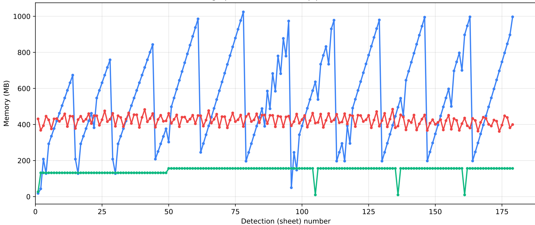
RAM usage per detection — CV pipeline (179 sheets)
