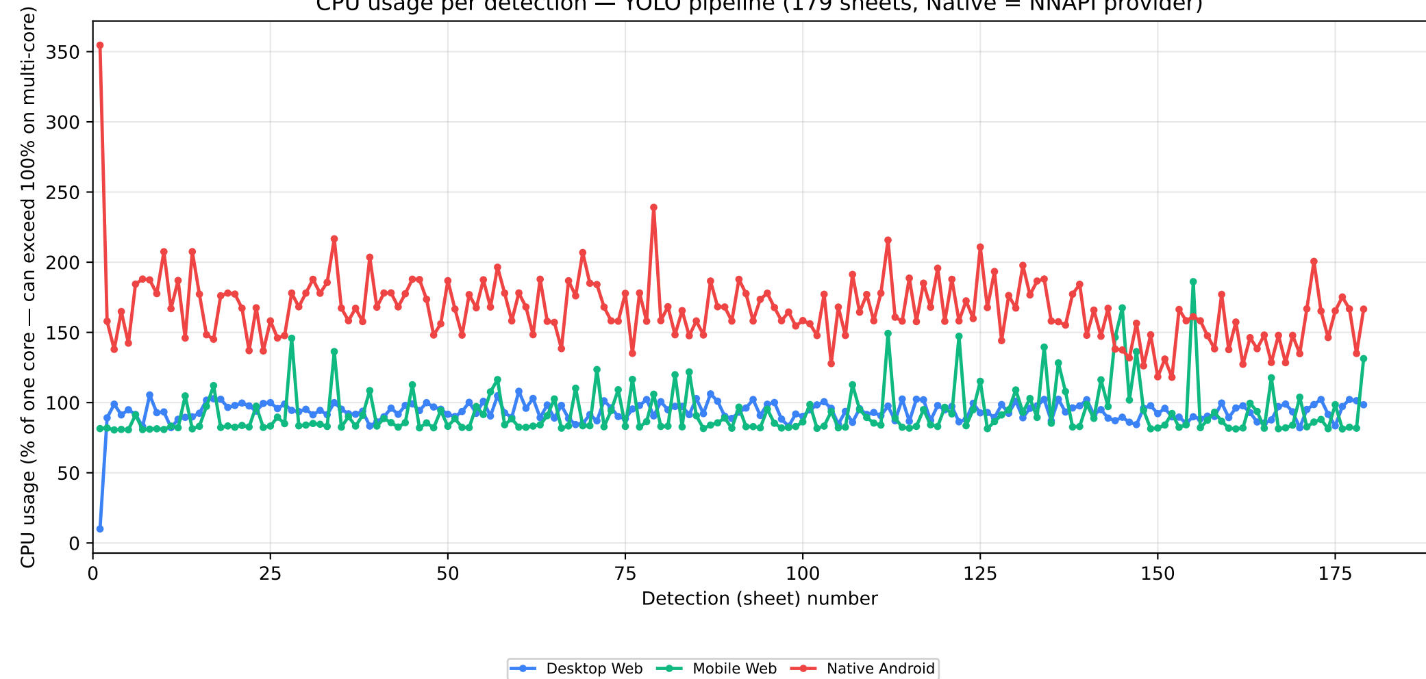
CPU usage per detection — YOLO pipeline (179 sheets, Native = NNAPI provider)
