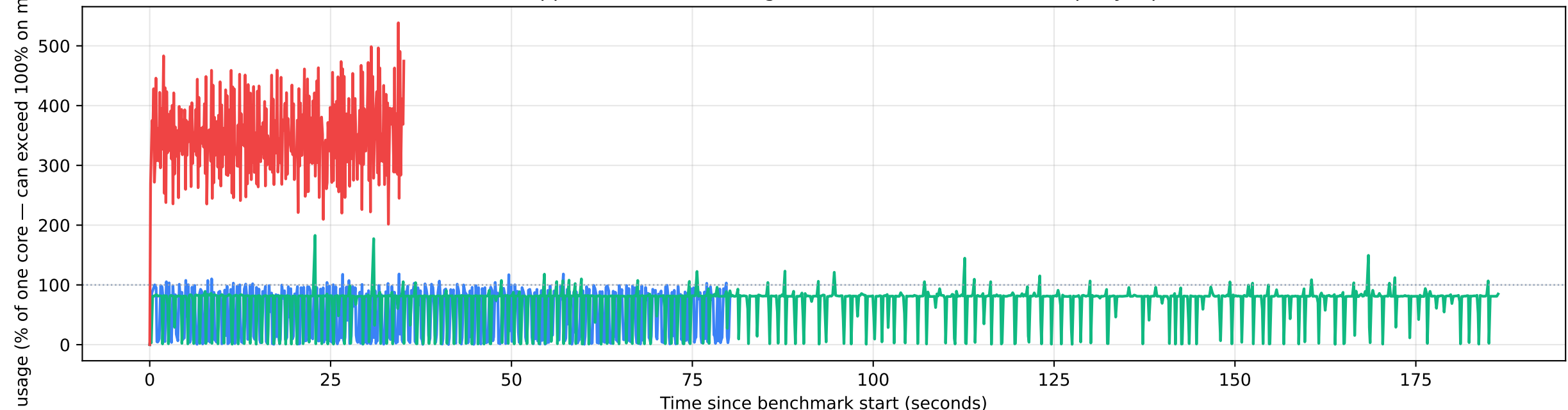
Process CPU utilisation over time — CV pipeline, harmonised plotting units Web: main-thread saturation × 100 (capped at ~100% — single-thread WASM) Native: top-style process CPU% (out of cores × 100)
