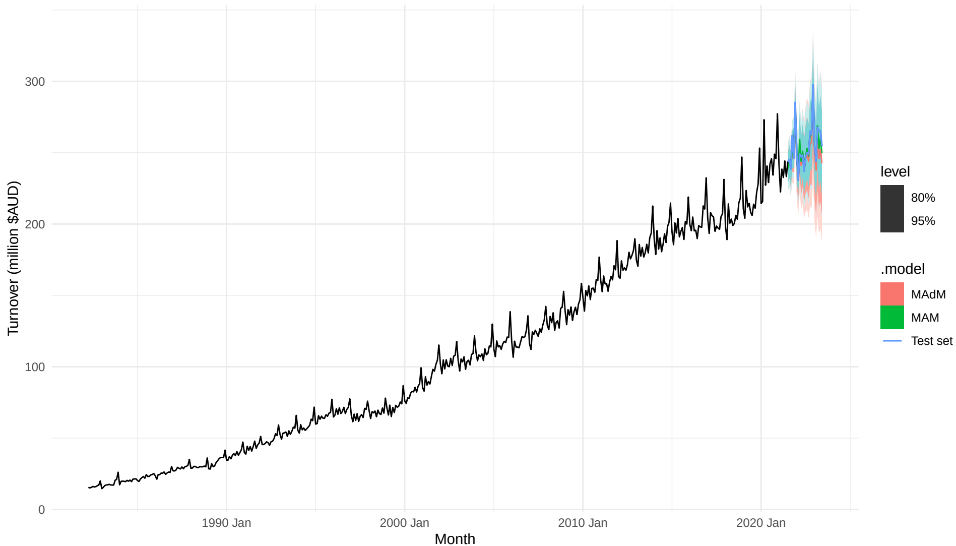
Forecasts for the last two years of the sample
