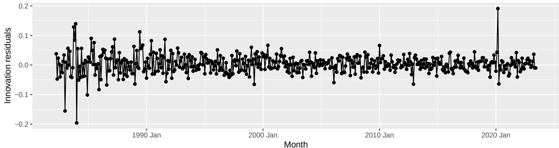
Residual diagnostics for ETS(M,Ad,M)
