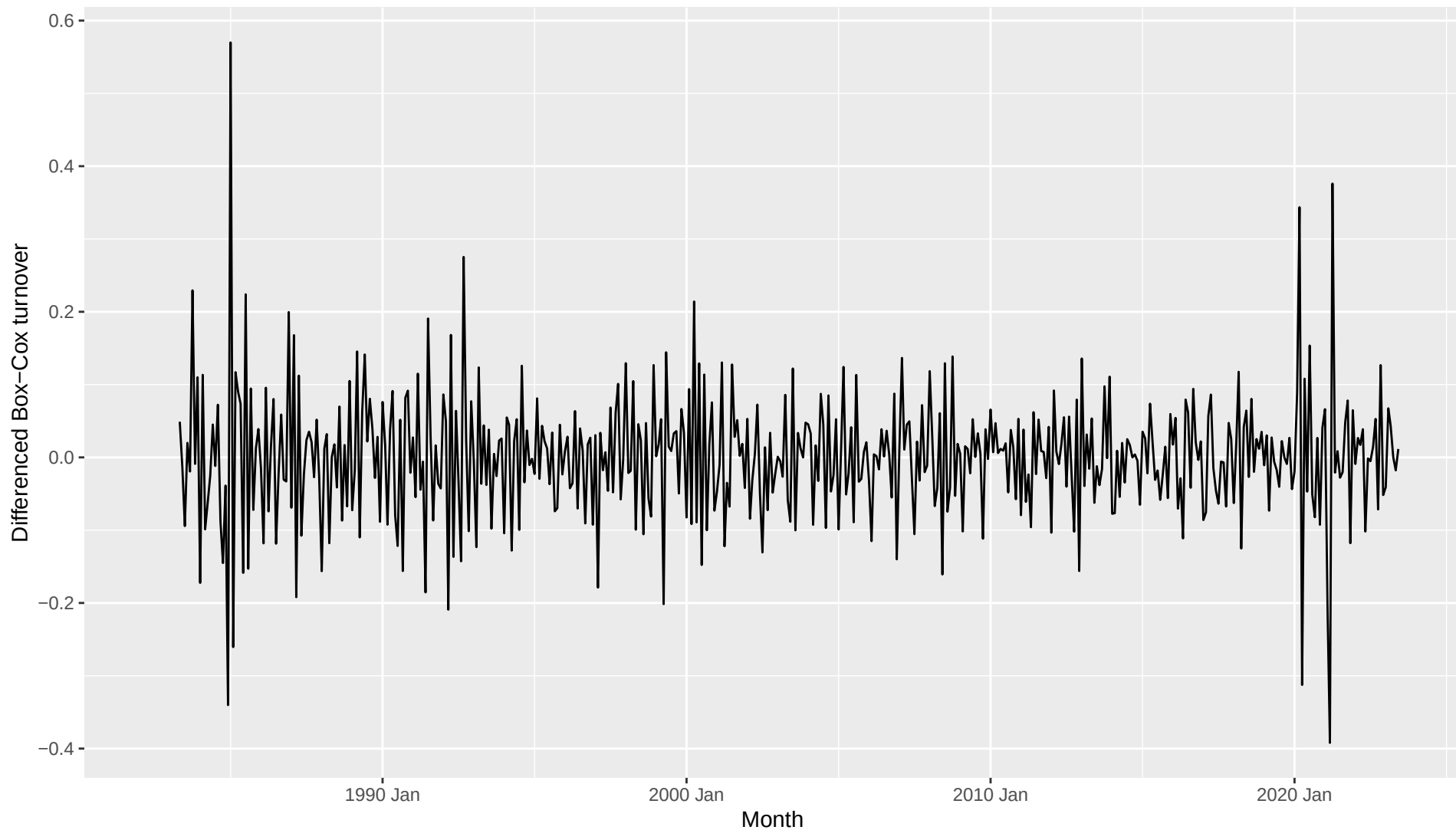
Seasonally and first differenced Box-Cox transformed series
