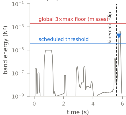
(a) slip episode, 100 Hz sensor
