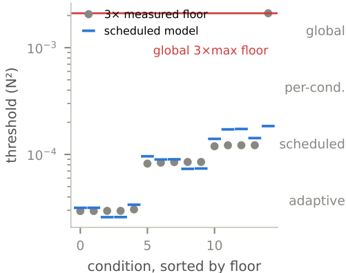
(b) 72\times floor spread
