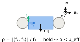
(b) grasp frame & utilization
