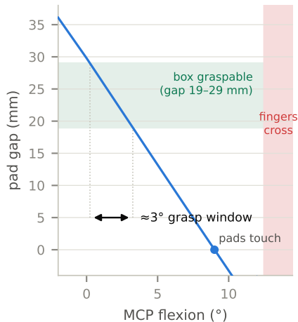
(c) thin grasp manifold ( \phi = 0, \theta = 0 )
