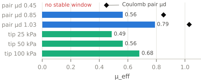
(b) material study — box, 50 g (blue: friction, teal: tip stiffness)
