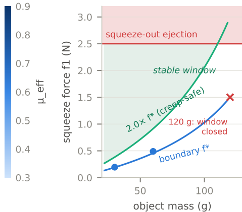
(c) force window, reference posture
