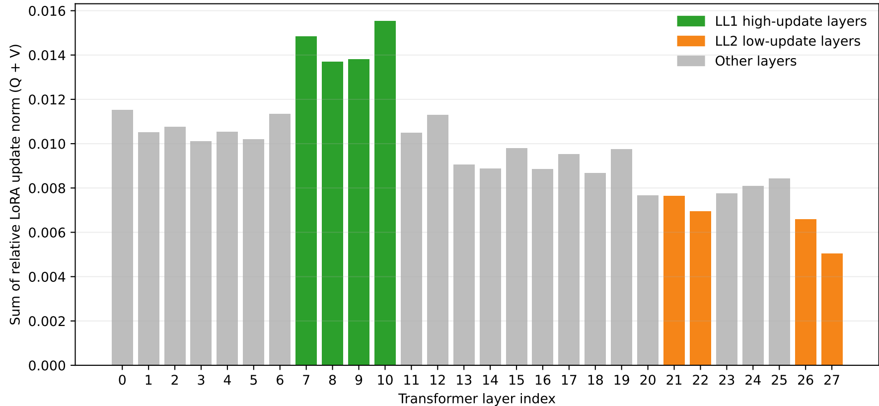
Layer-wise LoRA Update Scores for Selective-Layer Selection
