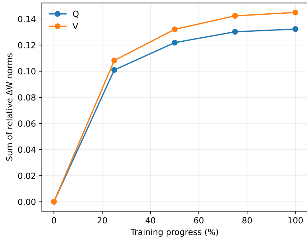
LoRA Update Growth, Module Allocation, and Validation Performance
