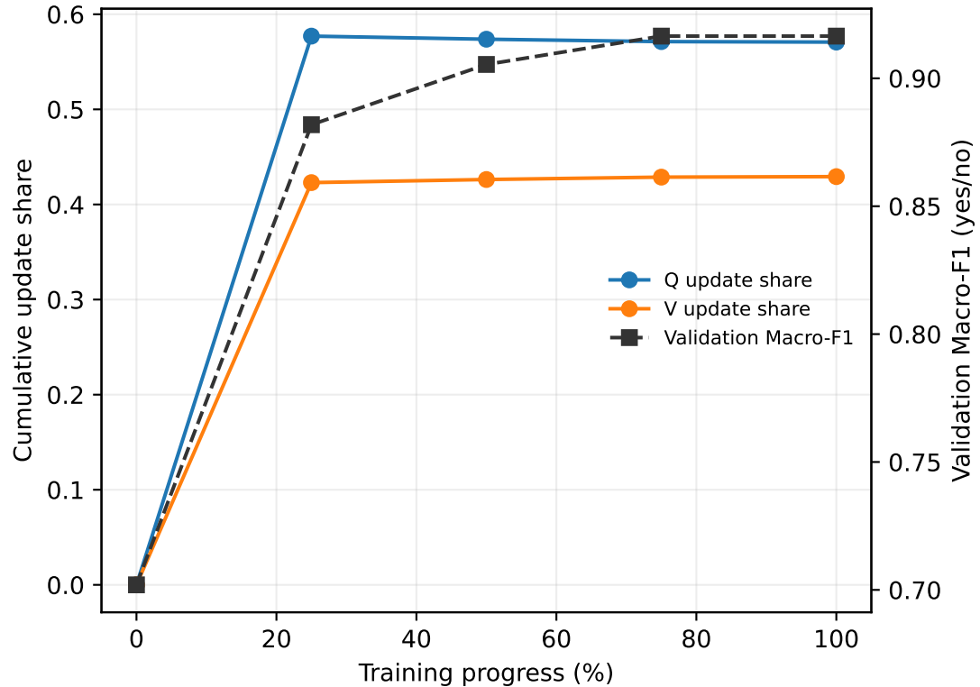
LoRA Update Growth, Module Allocation, and Validation Performance
