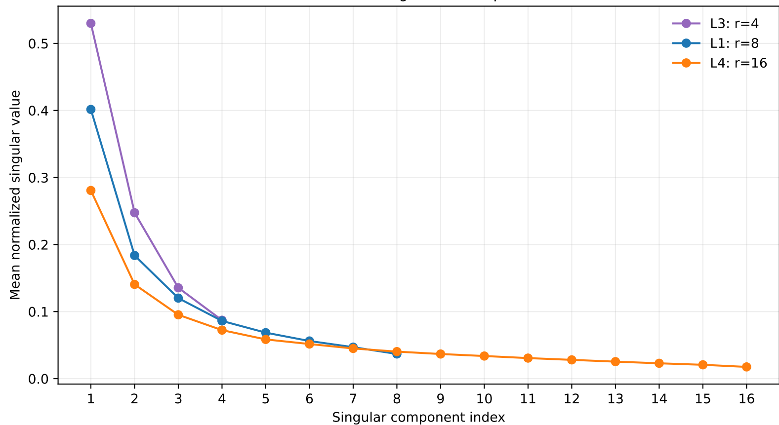
Final LoRA Singular-Value Spectra
